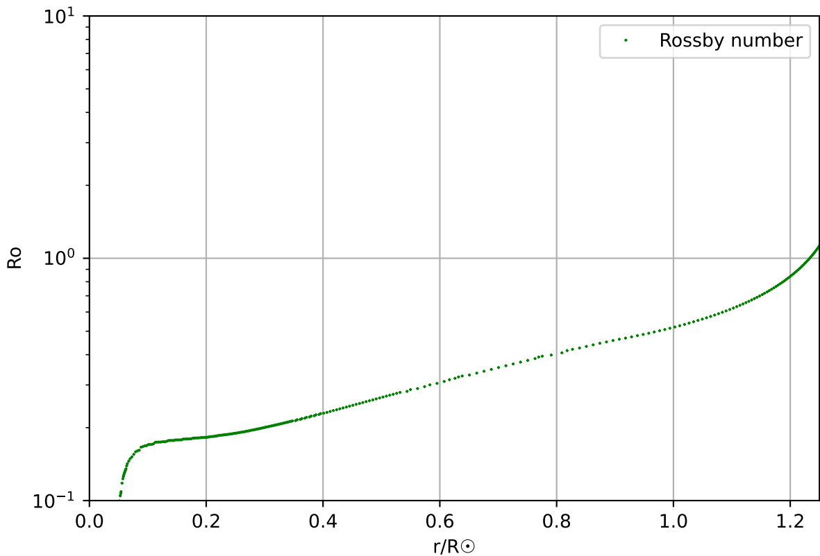
Rossby number, profile 171, age 9.97 \times 10^9
